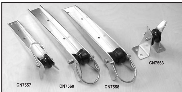
ANCHOR ROLLERS 304 Stainless Base with Black Urethane Roller
